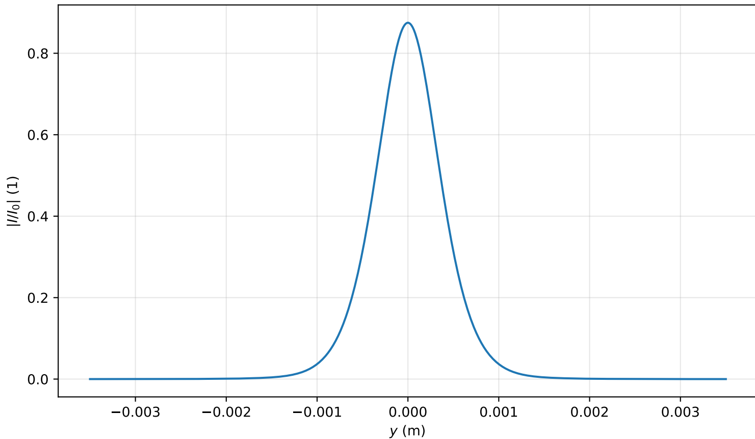
Intensity profile I(x=0, y, z=2.866)/I_0 , P_{in}=0.7P_{cr} , artificial time
